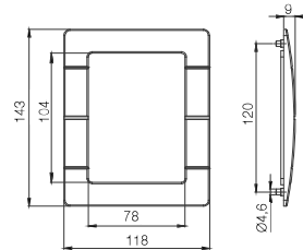
MP DWB800 / DWB1000 / DWB1600
