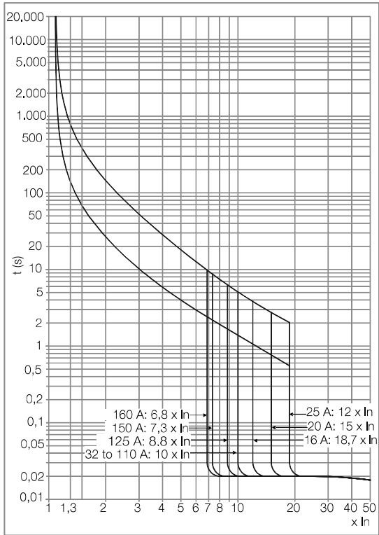
DWB160_M (Motor)
