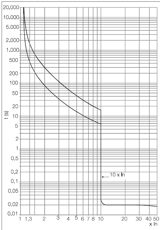
DWB250_M (Motor)
