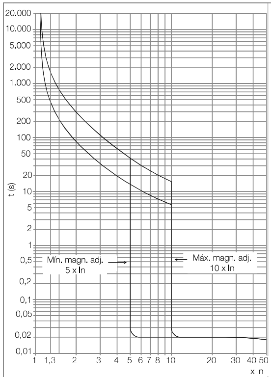
DWB400_M (Motor)
