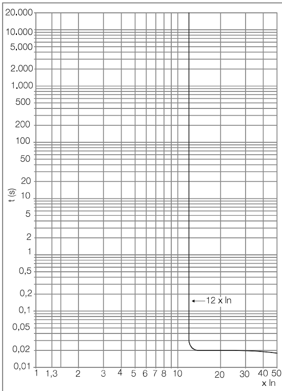
DWB160_M (Motor)
