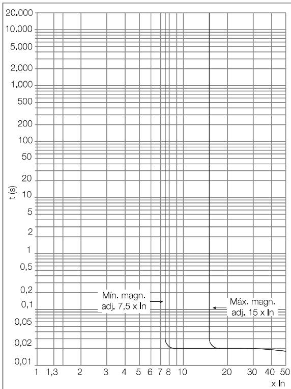
DWB800 (Motor)
