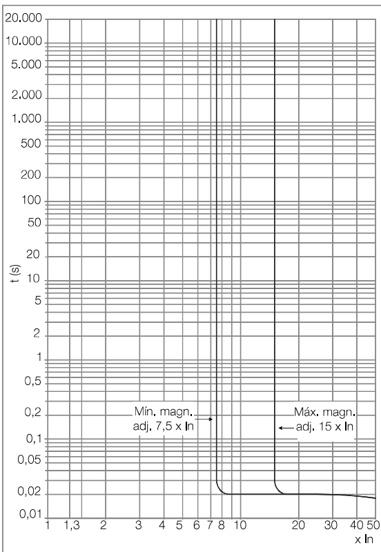
DWB400_M (Motor)
