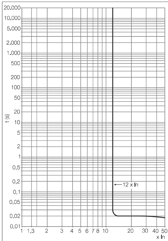
DWB250_M (Motor)
