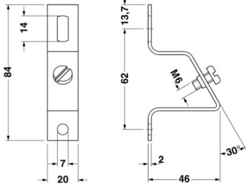
Dimensional drawing
